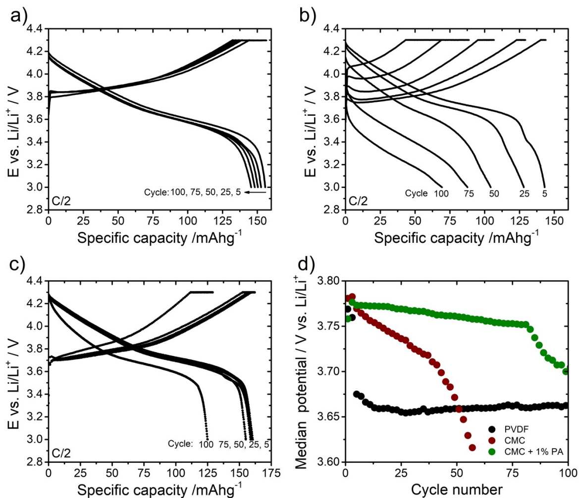
Figure S2. Capacity vs voltage for cycles 5, 25, 50, 75, and 100 of electrodes utilising binders of a) PVDF, b) CMC, and c) CMC+1%PA. Plot d) shows the evolution of the median discharge potential for these electrodes. Note that the data in c) is from "cell 2" as depicted in figure 1 of the main text.
