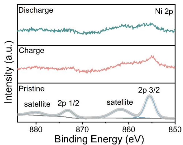
Fig. S22 Ex-situ Ni 2p XPS profiles of NMO cathode material in pristine, charge and discharge states.
