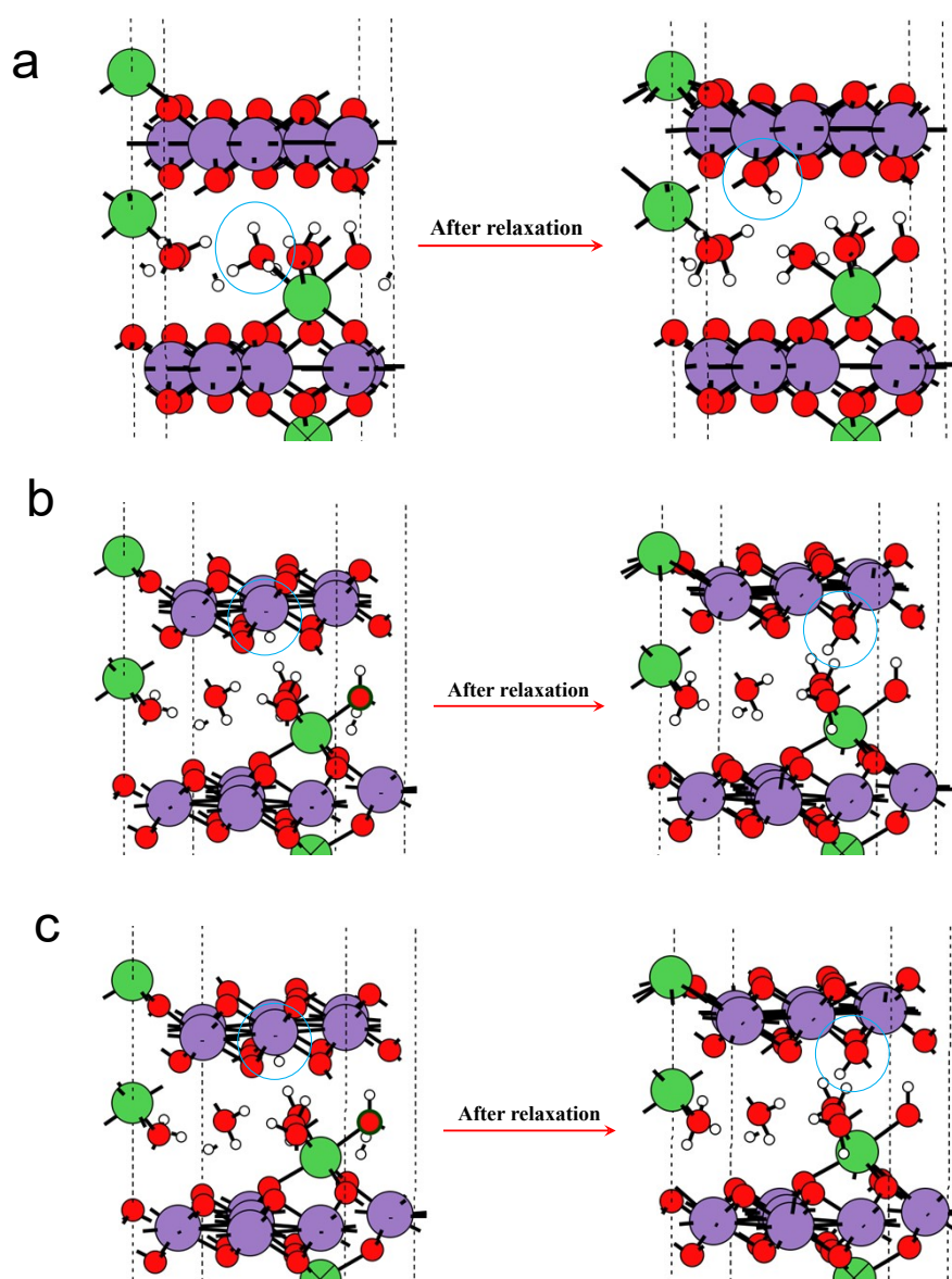
Fig. S15 Adsorption of proton (a) on inter-layer water molecules, (b) on \text{Mn}^{4+} ion and (c) on \text{O}^{2-} ions of the \text{NiMn}_3\text{O}_7 layer.
