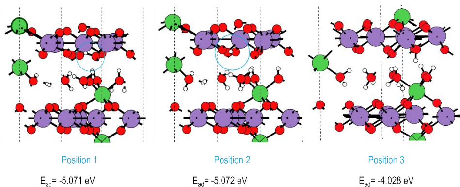
Fig.S17 Adsorption energies in different sites with an \text{Mn}^{4+} defect.
