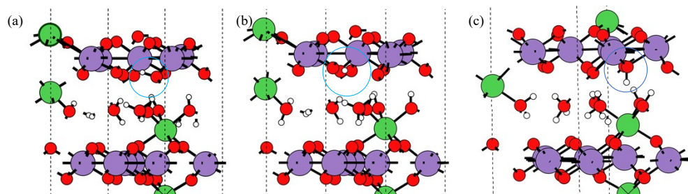
Fig.S16 Fully relaxed geometries of proton (a) on the \text{O}^{2-} ion, which migrated from the \text{Mn}^{4+} defect site, (b) on an \text{O}^{2-} ion next to the defect site, and (c) on an \text{O}^{2-} ion away from the \text{Mn}^{4+} defect site.
