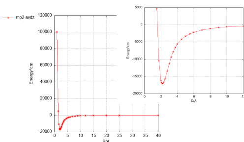
Fig. 4 \text{Ag}^+ -coronene complex interaction potential, evaluated at the MP2 level with aVDZ basis sets. See text for further details.
