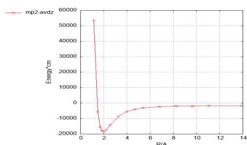
Fig. 5 \text{Ag}^+ -circumphyrene complex interaction potential, evaluated at the MP2 level with the aVDZ bases. See text for further details.
