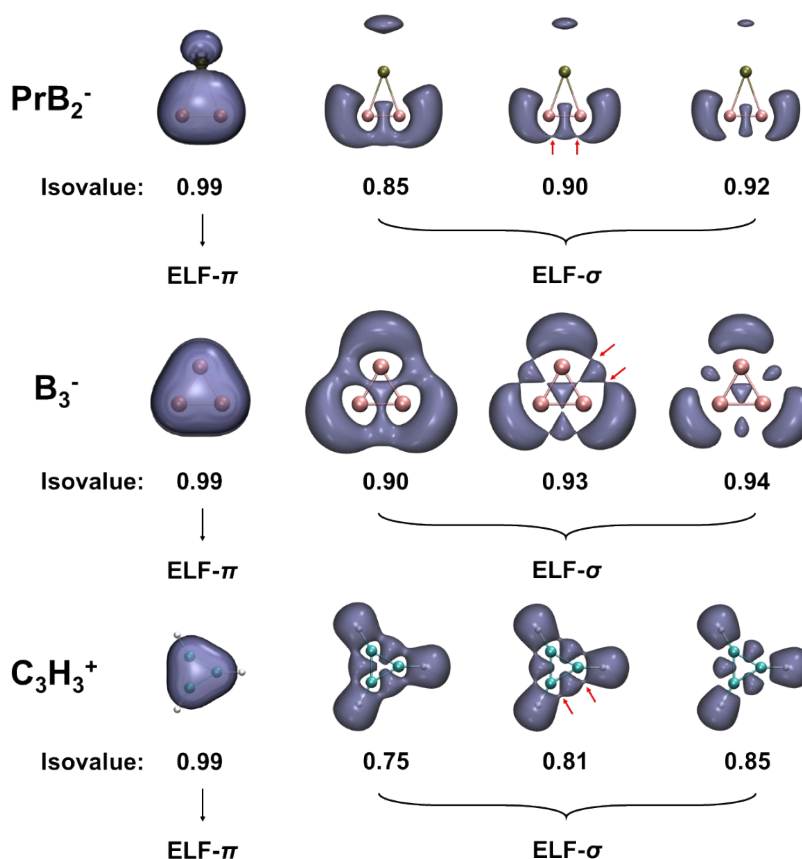
Figure S7. Results of bifurcation analysis of ELF- \sigma and ELF- \pi on \text{PrB}_2^- , \text{B}_3^- and \text{C}_3\text{H}_3^+ by using Gaussian 16 program. Some of the critical points are pointed out by red arrows; ELF- \pi do not have any reasonable critical points. Colour codes for atoms: olive – Pr; pink – B; cyan – C; white – H.
