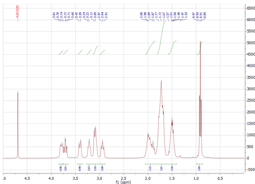
Fig. S2: ^1\text{H} NMR spectrum of the 7-ethyl-6-azoniaspiro[5.5]undecane (EASuD) bromide in \text{D}_2\text{O}
