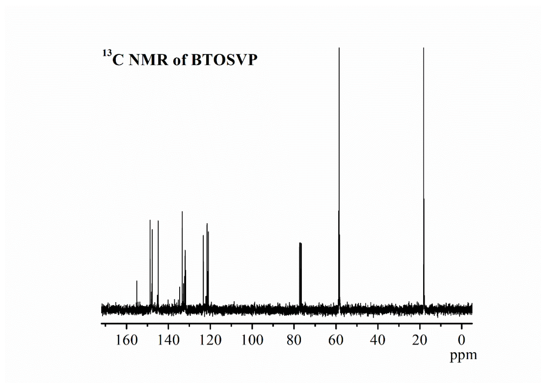
Figure S3. ^{13}\text{C} NMR spectras of 2,5-bis[(E)-2-(triethoxysilyl)vinyl]pyridine.
