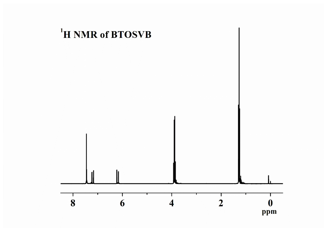
Figure S4. ^1\text{H} NMR spectras of 1,4-bis-((E)-2-(triethoxysilyl)vinyl)-benzene.
