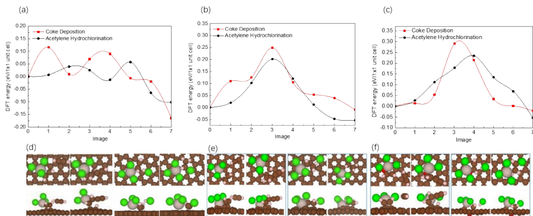
Fig S17. Minimum energy paths of acetylene polymerization ( C_2H_2 + C_2H_2 = C_4H_4 ) and acetylene hydrochlorination reactions on (a) RuCl 3 @graphene, (b) RuCl 3 @SV-O and (c) RuCl 3 @SV and the optimized initial and final structures of acetylene polymerization and acetylene hydrochlorination reactions on (d) RuCl 3 @graphene, (e) RuCl 3 @SV-O and (f) RuCl 3 @SV.
