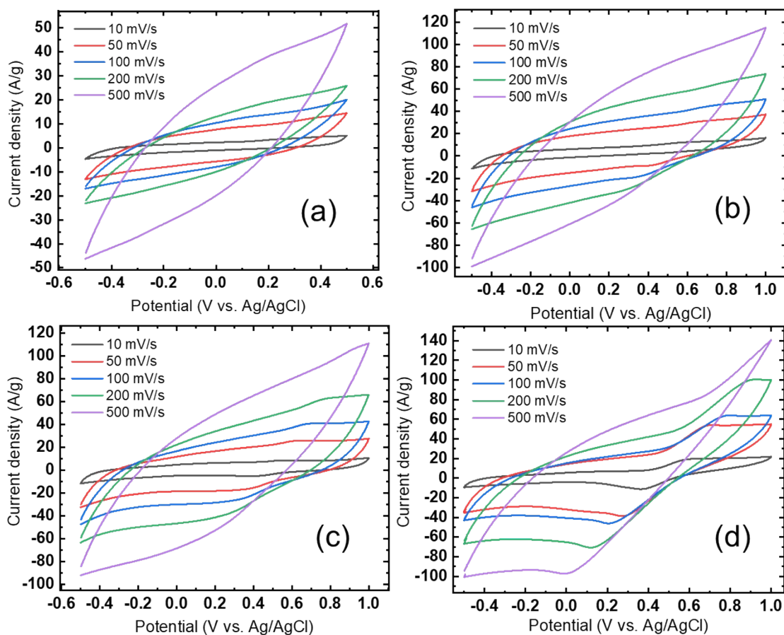
Figure S7. CV of (a) GM0, (b) GM1, (c) GM2, and (d) GM3 at different scan rates. The CV plots show appearance of redox peak with higher \text{Ti}_3\text{C}_2\text{T}_z content (GM2 and GM3). At high scan rate the CV nature of GM2 is stable but GM3 got distorted due to excess \text{Ti}_3\text{C}_2\text{T}_z content.
