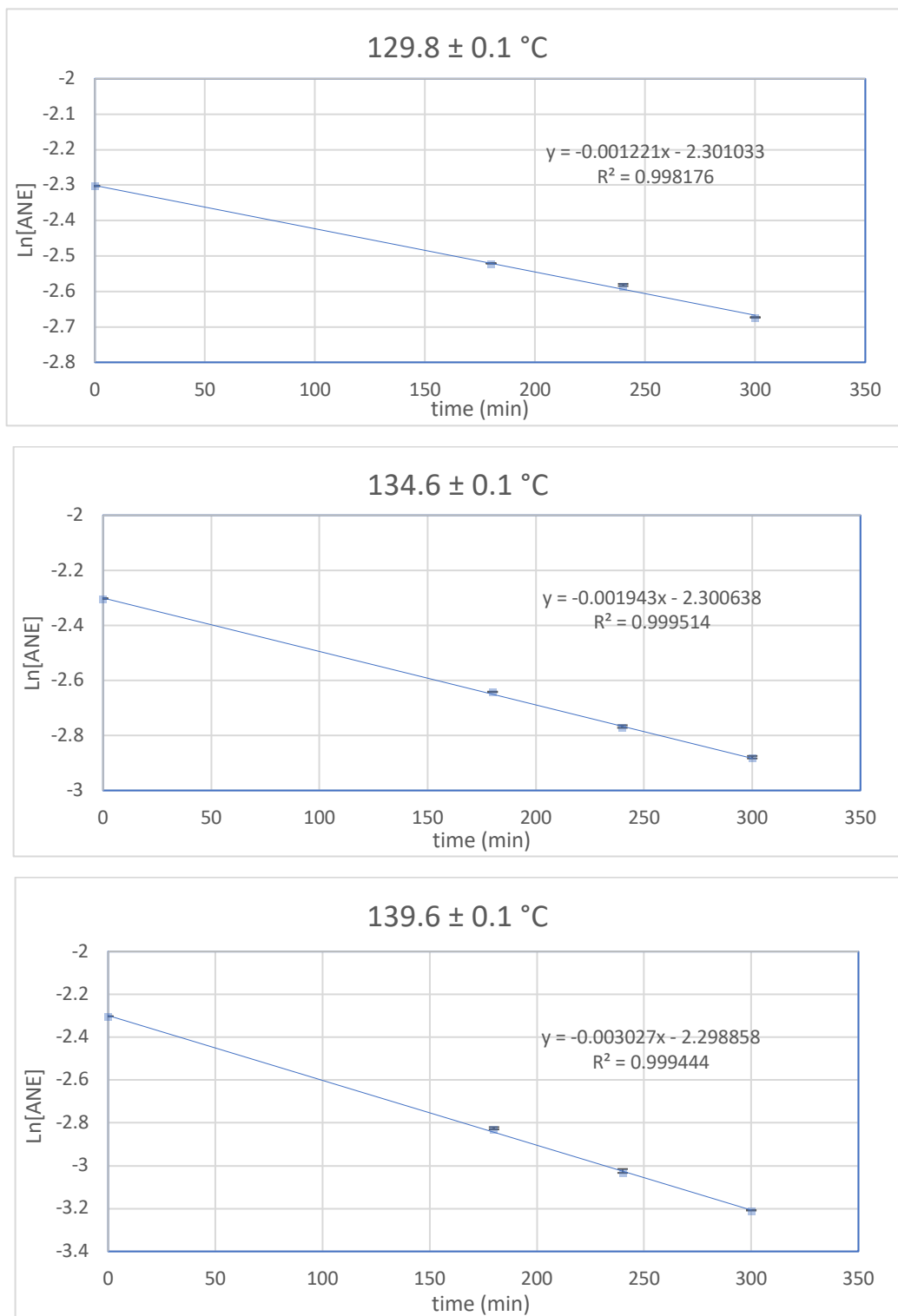
Figure S4. Plots of \text{Ln}[\text{ANE}] against time to obtain rate constants at various temps
