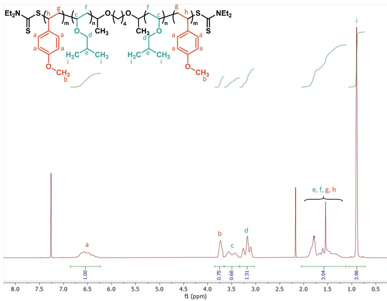
Figure S10.3: Quantitative ^1\text{H} NMR of PMOS-0.32 in \text{CDCl}_3
