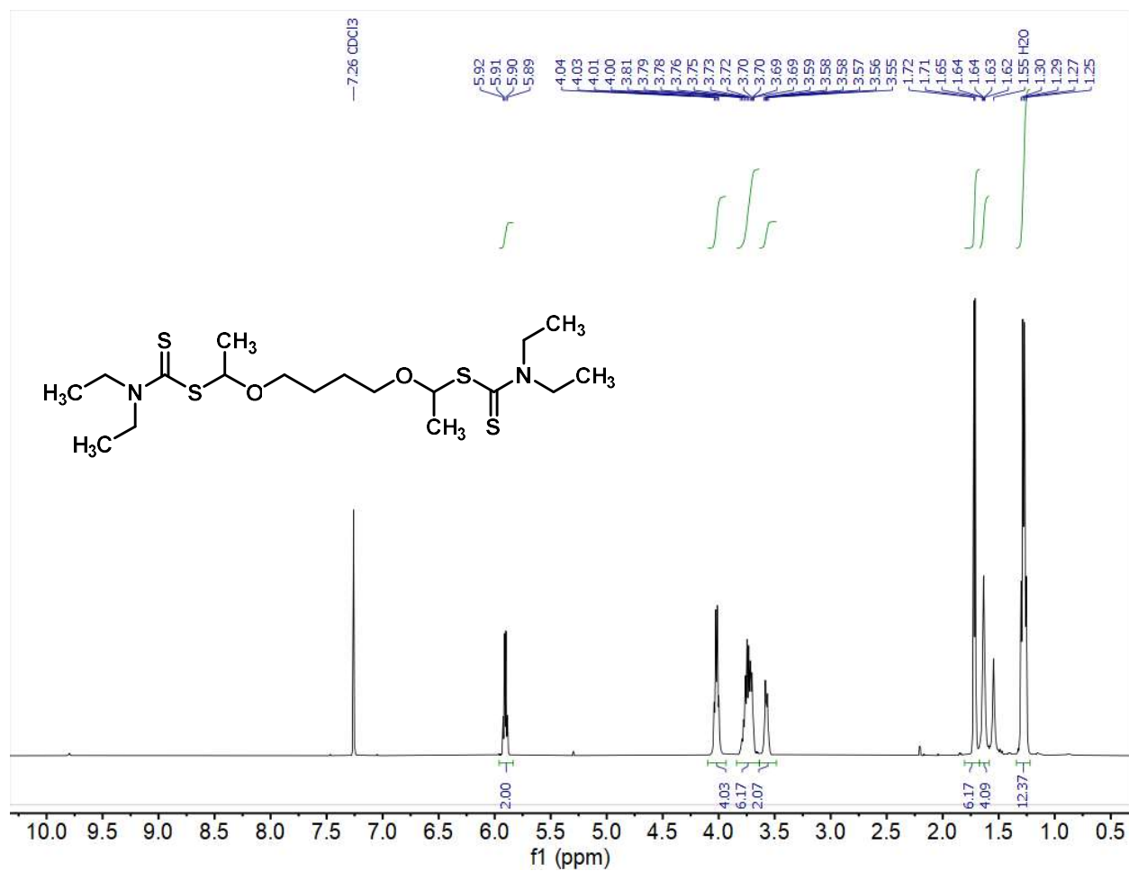
Figure S9.1: Quantitative ^1\text{H} NMR of difunctional CTA in CDCl 3
