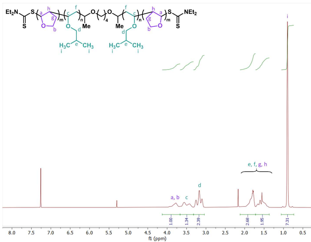
Figure S10.5: Quantitative ^1\text{H} NMR of PDHF-0.23 in CDCl 3
