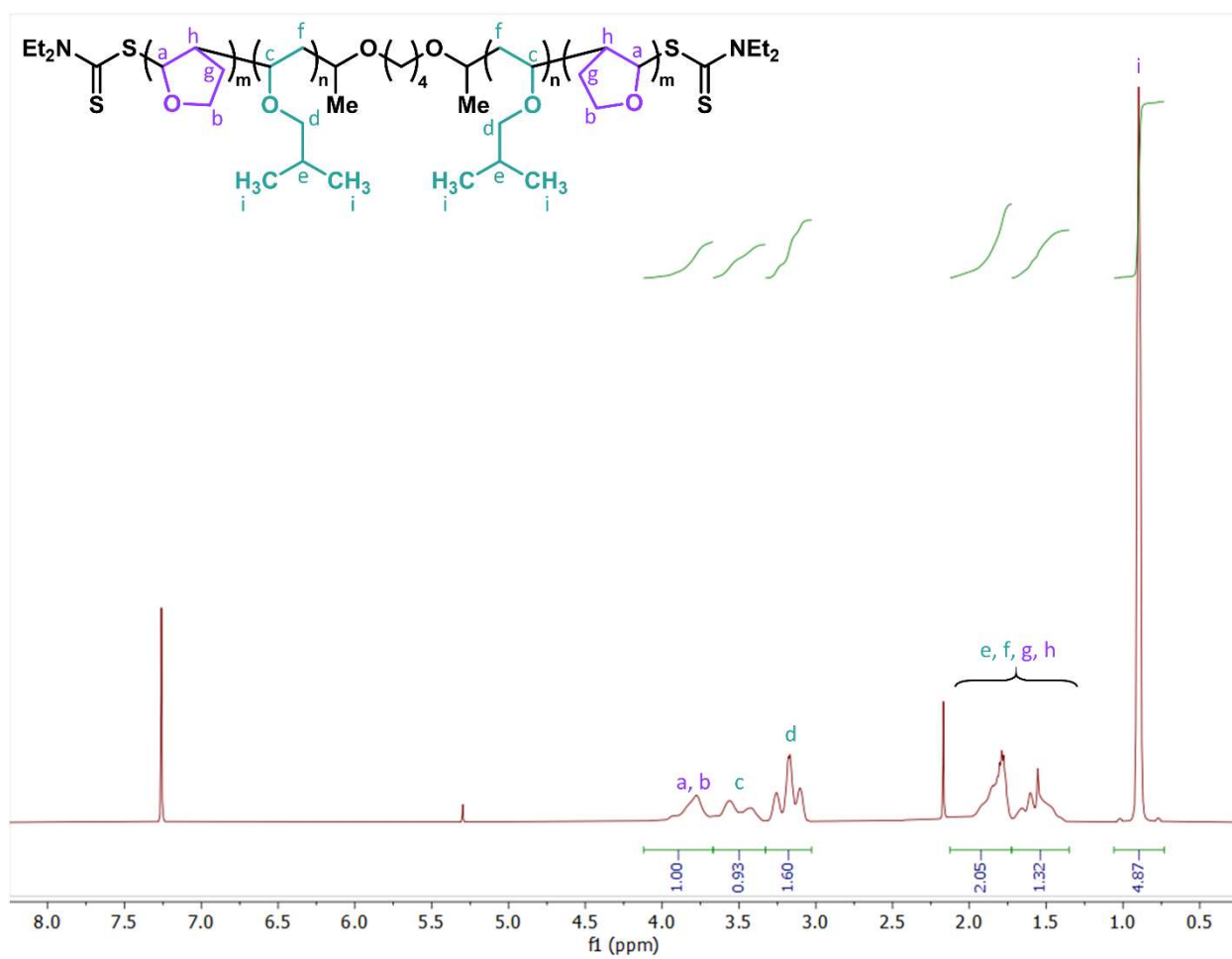
Figure S10.6: Quantitative ^1\text{H} NMR of PDHF-0.31 in \text{CDCl}_3
