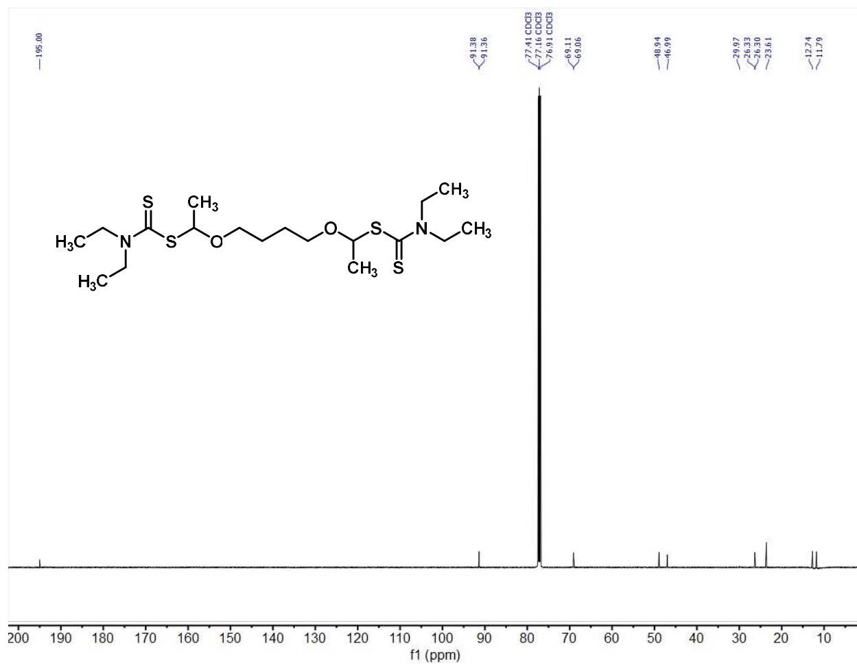
Figure S9.2: ^{13}\text{C} NMR of Difunctional CTA in \text{CDCl}_3
