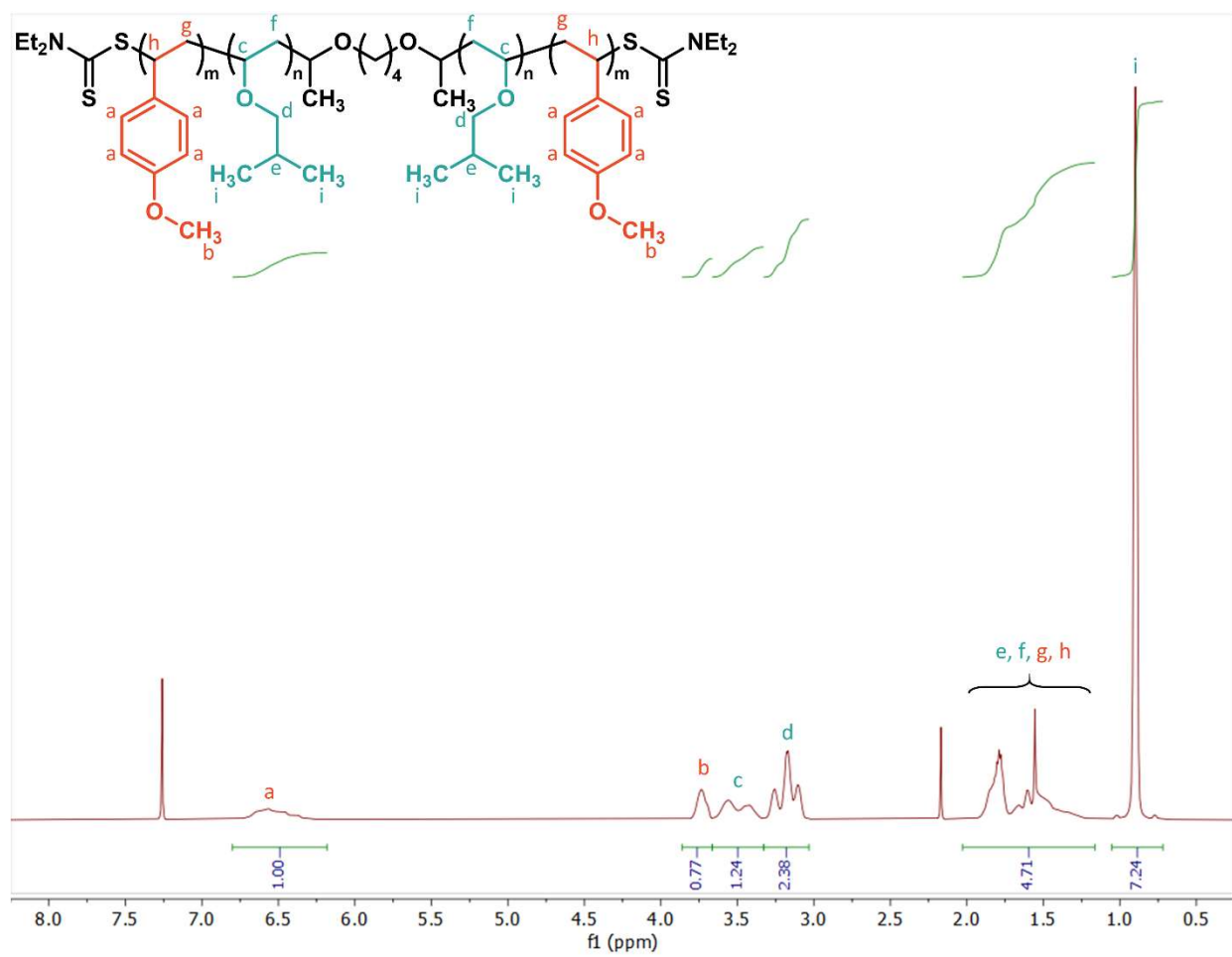
Figure S10.1: Quantitative ^1\text{H} NMR of PMOS-0.21 in \text{CDCl}_3
