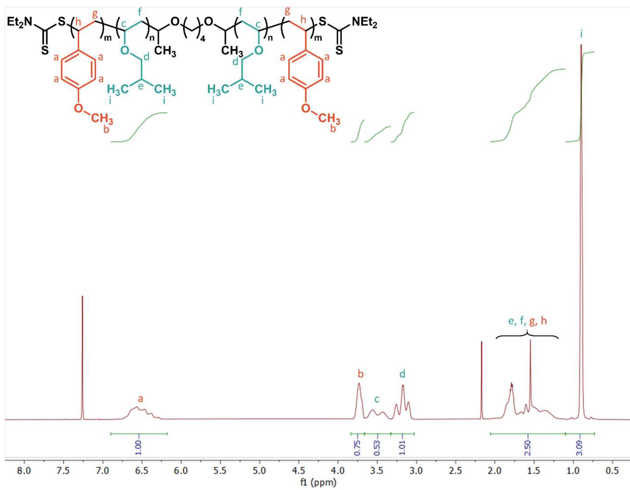
Figure S10.4: Quantitative ^1\text{H} NMR of PMOS-0.38 in \text{CDCl}_3
