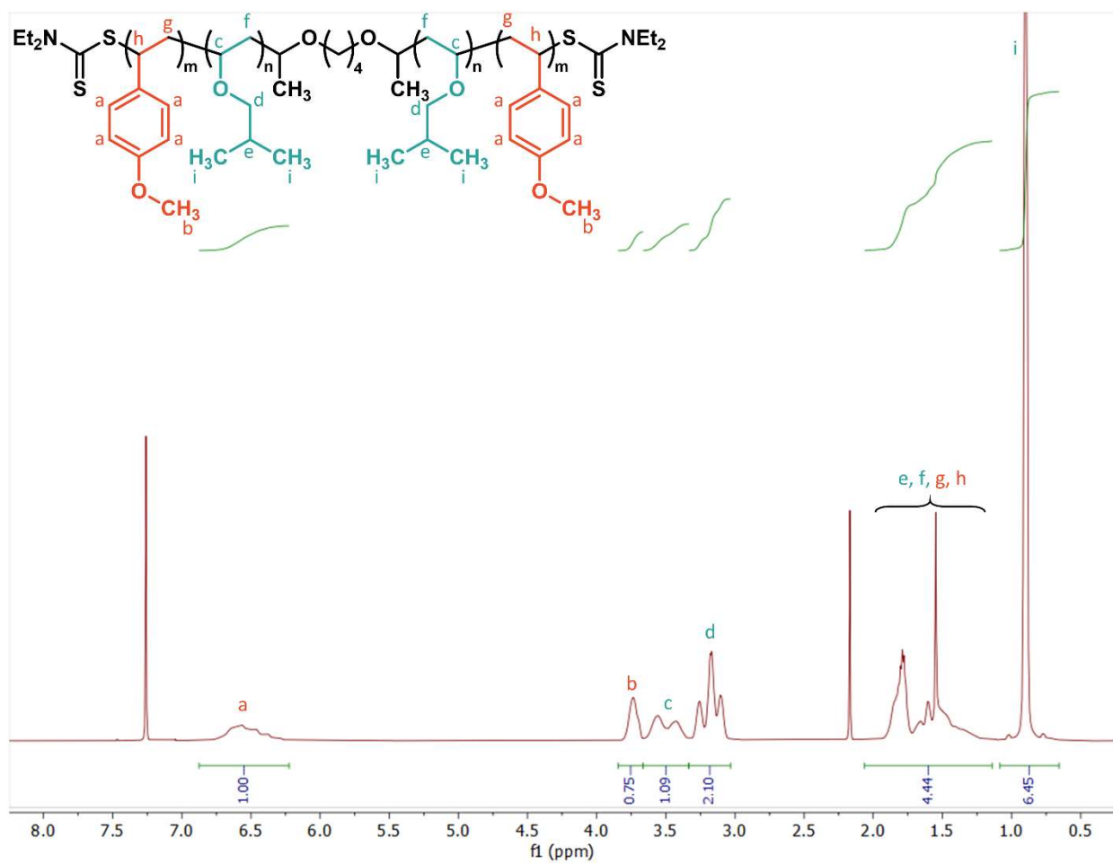
Figure S10.2: Quantitative ^1\text{H} NMR of PMOS-0.23 in \text{CDCl}_3
