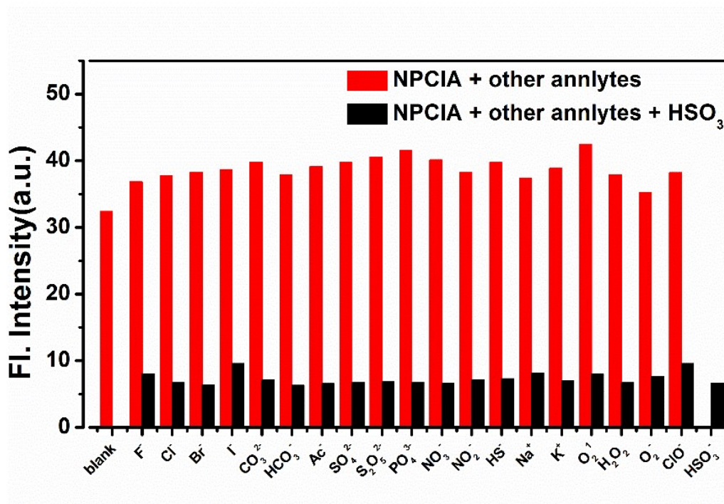
Fig. S9 Changes in fluorescence of NPCIA (10 \mu M) at 585 nm with HSO 3 - (100 \mu M) and other analytes (100 \mu M of Na + , K + , F - , Cl - , Br - , I - , CO 3 2- , HCO 3 - , Ac - , SO 4 2- , PO 4 3- , S 2 O 5 2- , HS - , NO 3 - , NO 2 - , NO•, O 2 • - , 1 O 2 , ClO - and H 2 O 2 ). Conditions: \lambda_{\text{ex}} = 544 nm. Slit: 10/10 nm.
