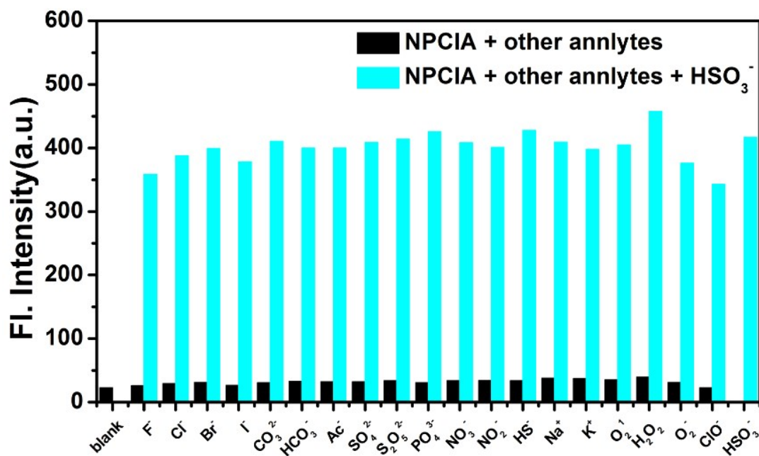
Fig. S8 Changes in fluorescence of NPCIA (10 \mu\text{M} ) at 482 nm with \text{HSO}_3^- (100 \mu\text{M} ) and other analytes (100 \mu\text{M} of \text{Na}^+ , \text{K}^+ , \text{F}^- , \text{Cl}^- , \text{Br}^- , \text{I}^- , \text{CO}_3^{2-} , \text{HCO}_3^- , \text{Ac}^- , \text{SO}_4^{2-} , \text{PO}_4^{3-} , \text{S}_2\text{O}_5^{2-} , \text{HS}^- , \text{NO}_3^- , \text{NO}_2^- , \text{NO}\cdot , \text{O}_2\cdot^- , ^1\text{O}_2 , \text{ClO}^- and \text{H}_2\text{O}_2 ). Conditions: \lambda_{\text{ex}} = 395 \text{ nm} . Slit: 10/10 nm.
