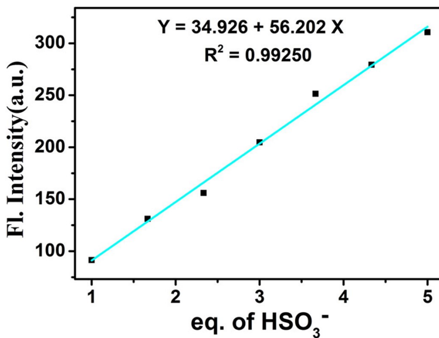
Fig.S5 A linear relationship between the fluorescence intensity of NPCIA and HSO 3 - (1-5 equiv.). Conditions: \lambda_{\text{ex}} = 395 nm, \lambda_{\text{em}} = 482 nm. Slit: 10/10 nm.
