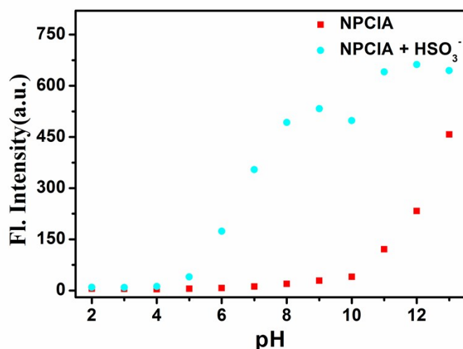
Fig. S12 The pH effect of the test solution on NPCIA (10 \mu\text{M} ) was tested in the absence or presence of \text{HSO}_3^- (10 equiv.). Conditions: \lambda_{\text{ex}} = 395 \text{ nm} , \lambda_{\text{em}} = 482 \text{ nm} . Slit: 10/10 nm.
