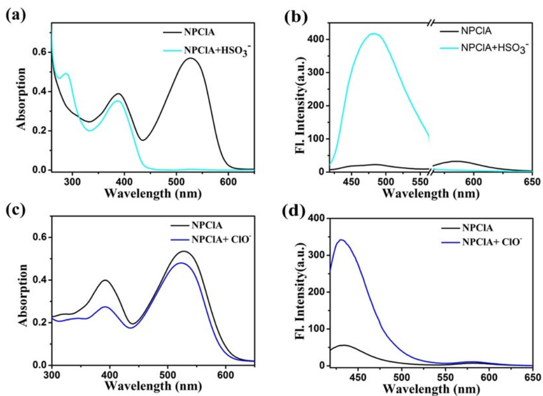
Fig. S4 (a and c) Absorption and (b and d) fluorescence emission spectra of NPCIA for recognizing \text{HSO}_3^- and \text{ClO}^- . (b) \lambda_{\text{ex}} = 395 \text{ nm} , \lambda_{\text{em}} = 482 \text{ nm} ; \lambda_{\text{ex}} = 544 \text{ nm} , \lambda_{\text{em}} = 585 \text{ nm} . (d) \lambda_{\text{ex}} = 395 \text{ nm} , \lambda_{\text{em}} = 425 \text{ nm} . Slit: 10/10 nm.
