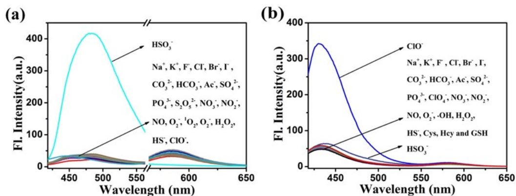
Fig. S7 (a) Changes in fluorescence of NPCIA (10 \mu\text{M} ) with \text{HSO}_3^- (100 \mu\text{M} ) and other analytes (100 \mu\text{M} of \text{Na}^+ , \text{K}^+ , \text{F}^- , \text{Cl}^- , \text{Br}^- , \text{I}^- , \text{CO}_3^{2-} , \text{HCO}_3^- , \text{Ac}^- , \text{SO}_4^{2-} , \text{PO}_4^{3-} , \text{S}_2\text{O}_5^{2-} , \text{HS}^- , \text{NO}_3^- , \text{NO}_2^- , \text{NO}\cdot , \text{O}_2\cdot^- , ^1\text{O}_2 , \text{ClO}^- and \text{H}_2\text{O}_2 ). (b) Changes in fluorescence of NPCIA (10 \mu\text{M} ) with \text{ClO}^- (100 \mu\text{M} ) and other analytes (100 \mu\text{M} of \text{Na}^+ , \text{K}^+ , \text{F}^- , \text{Cl}^- , \text{Br}^- , \text{I}^- , \text{CO}_3^{2-} , \text{HCO}_3^- , \text{Ac}^- , \text{SO}_4^{2-} , \text{PO}_4^{3-} , \text{ClO}_4^- , \text{HS}^- , \text{HSO}_3^- , Cys, Hcy, GSH, \text{NO}_3^- , \text{NO}_2^- , \cdot\text{OH} , \text{NO}\cdot , \text{O}_2\cdot^- and \text{H}_2\text{O}_2 ). Conditions: (a) \lambda_{\text{ex}} = 395 \text{ nm} , \lambda_{\text{em}} = 482 \text{ nm} ; \lambda_{\text{ex}} = 544 \text{ nm} , \lambda_{\text{em}} = 585 \text{ nm} . (b) \lambda_{\text{ex}} = 395 \text{ nm} , \lambda_{\text{em}} = 425 \text{ nm} . Slit: 10/10 nm.
