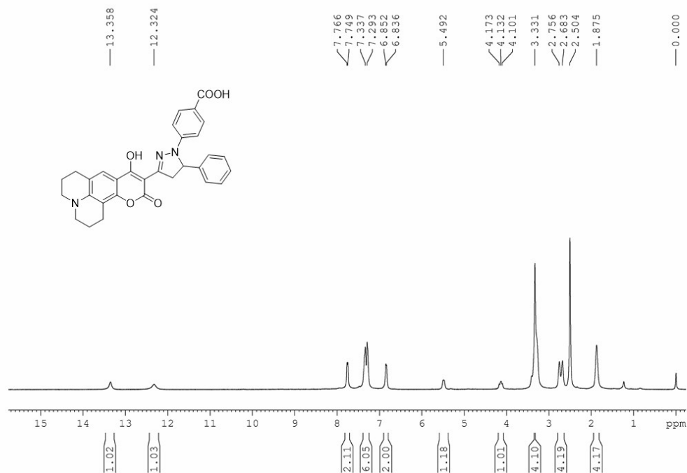
^1\text{H} -NMR spectrum of compound 3 in \text{DMSO}-d_6
