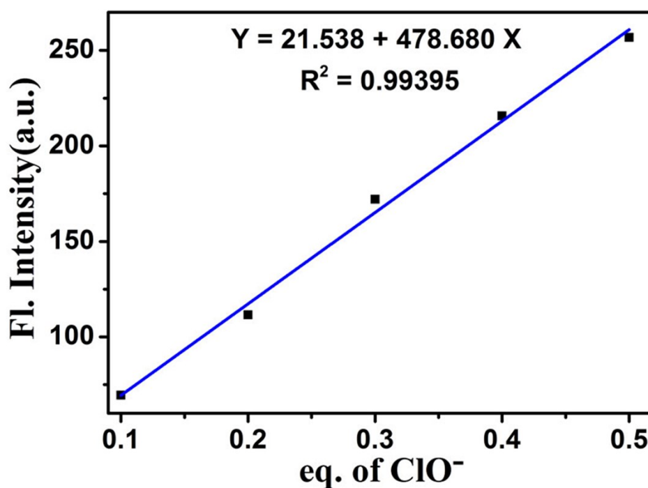
Fig.S6 A linear relationship between the fluorescence intensity of NPCIA and ClO - (0.1-0.5 equiv.). Conditions: \lambda_{\text{ex}} = 395 nm, \lambda_{\text{em}} = 425 nm. Slit: 10/10 nm.
