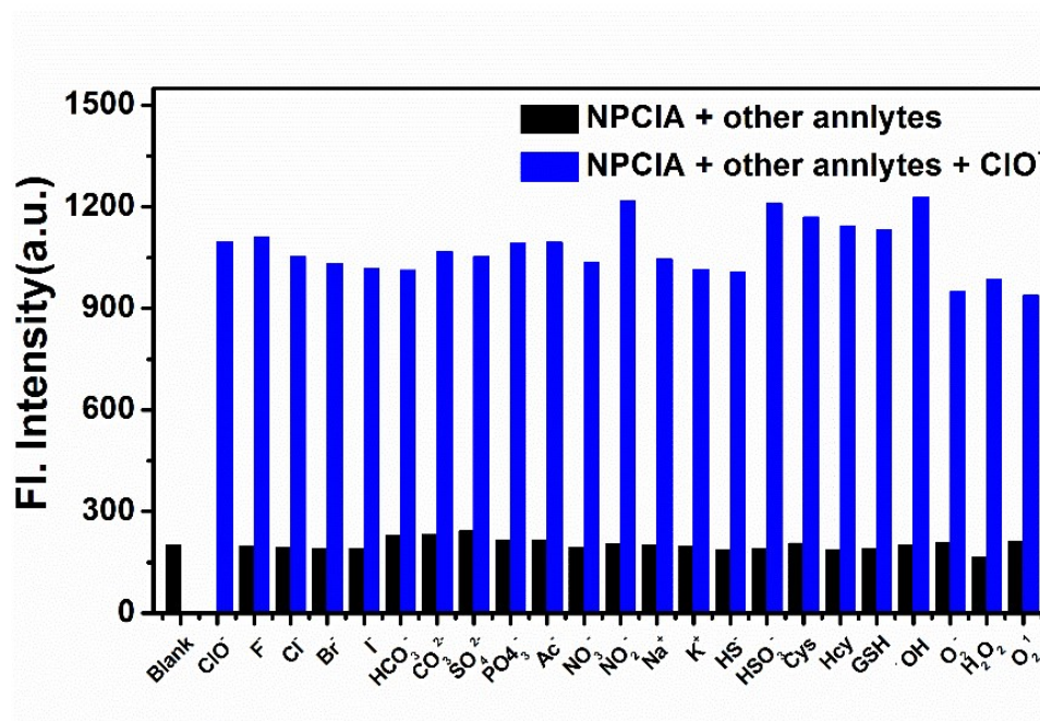
Fig. S10 Changes in fluorescence of NPCIA (10 \mu M) with ClO - (100 \mu M) and other analytes (100 \mu M of Na + , K + , F - , Cl - , Br - , I - , CO 3 2- , HCO 3 - , Ac - , SO 4 2- , PO 4 3- , ClO 4 - , HS - , HSO 3 - , Cys, Hcy, GSH, NO 3 - , NO 2 - , •OH, NO•, O 2 • - and H 2 O 2 ). Conditions: \lambda_{\text{ex}} = 395 nm, \lambda_{\text{em}} = 425 nm. Slit: 10/10 nm.
