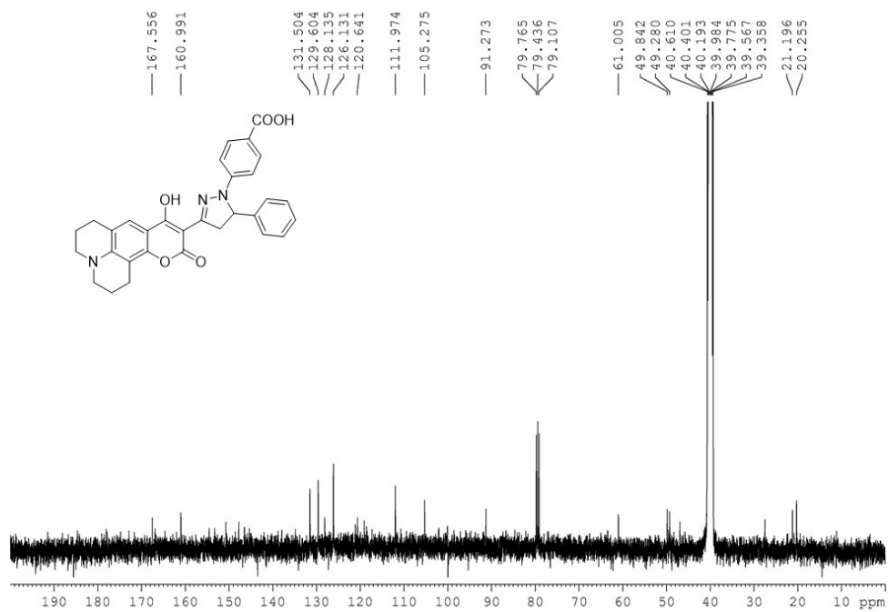
^{13}\text{C} -NMR spectrum of compound 3 in \text{DMSO}-d_6
