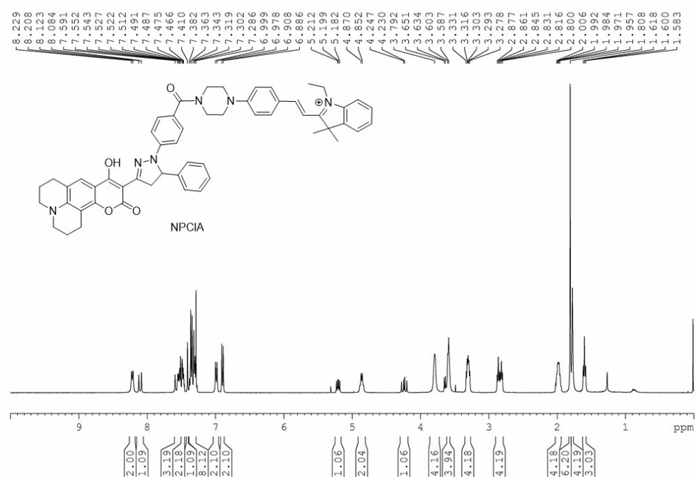
^1\text{H} -NMR spectrum of probe NPCIA in \text{CDCl}_3
