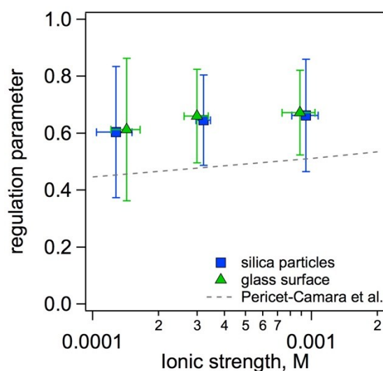
Figure S3-1: Determined regulation parameter as a function of the fitted total ionic strength for silica (blue squares) and glass surfaces (green triangles). The dashed line are the theoretical calculations by Pericet-Camara et al. 1
