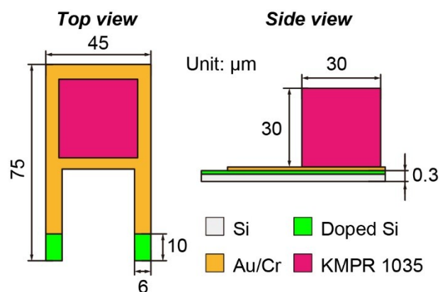
Figure S1 Design parameters of a piezoresistive cantilever.
